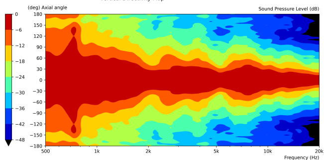
Vertical Directivity Map
