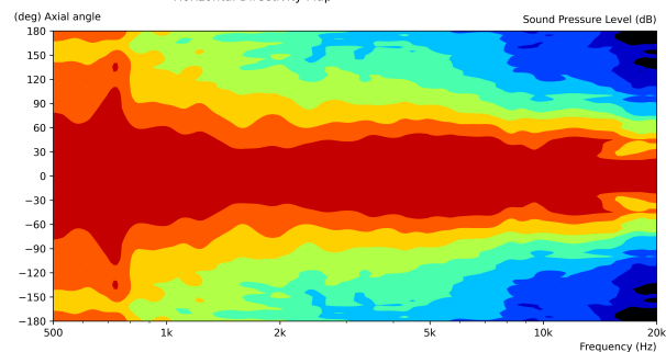
Horizontal Directivity Map
