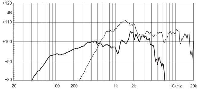
FREQUENCY RESPONSE CURVE OF 15CX1000 MADE ON 125 LT ENCLOSURE TUNED 50HZ IN FREE FIELD (4PI) ENVIRONMENT. ENCLOSURE CLOSES THE REAR OF THE DRIVER. THIN LINE REPRESENTS HIGH FREQUENCY RESPONSE.
