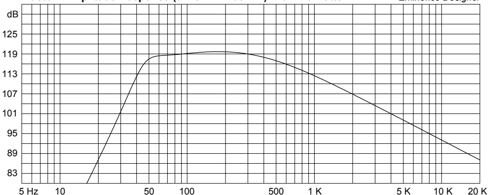
Custom Amplitude Response (dB-SPL/Hz at 1 m) with 175 watts
